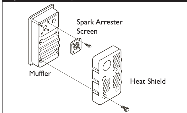
Figure 12 — Service Spark Arrester
